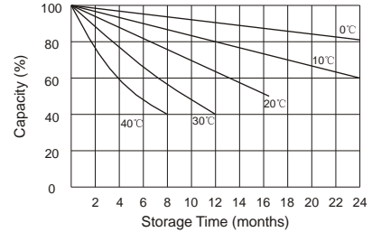
Self-discharge characteristic
