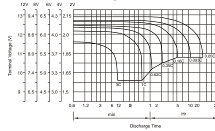
Discharge characteristic Curve
