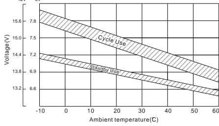
Relationship between charging voltage and temperature
